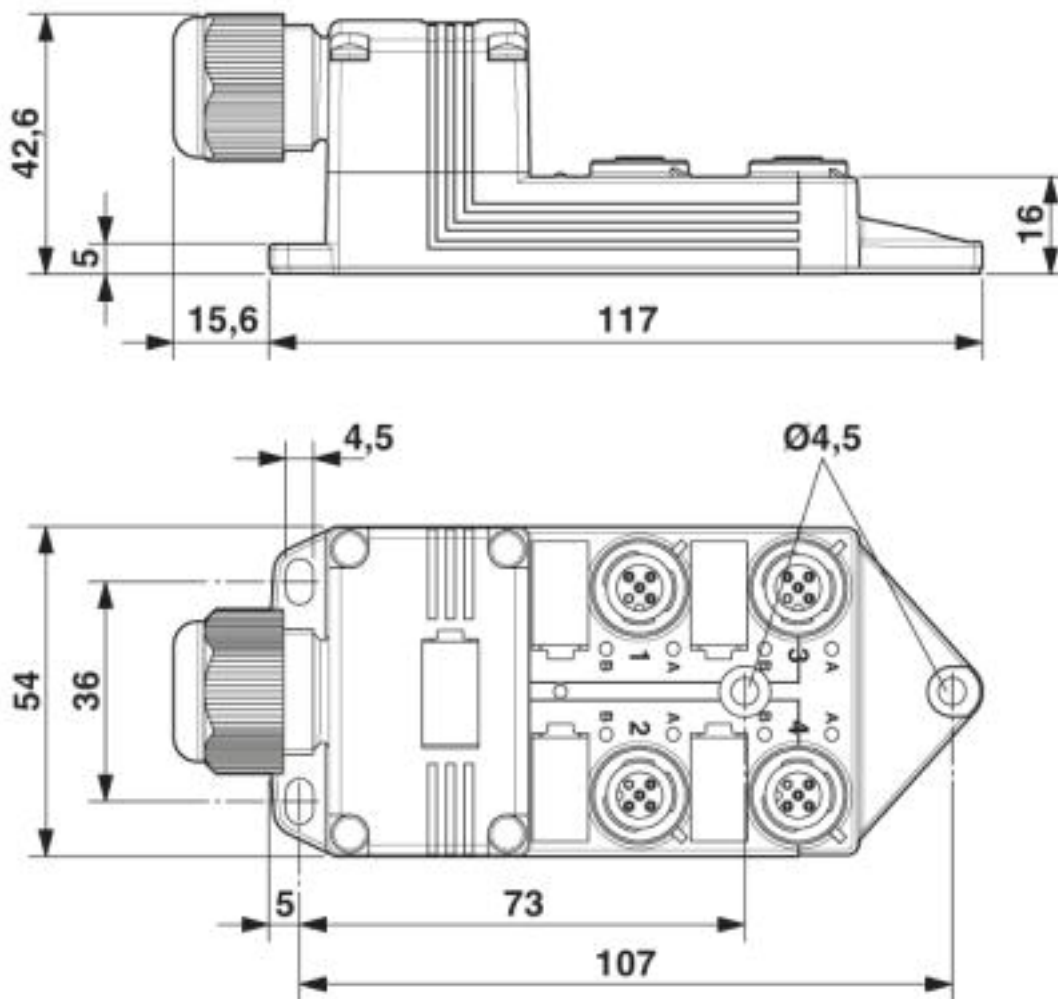
Dimensioned drawing
