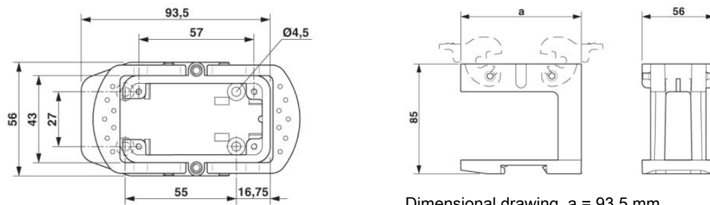
Dimensional drawing top view
