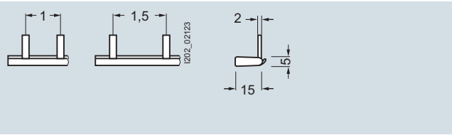
5ST3701-0HG 5ST3703-0HG
