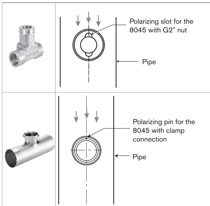
Fig. 8: Installing a T fitting
