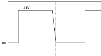
Latency of power sink equipped power supply
