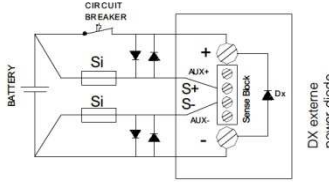
External Sense Protection (fig.8)
