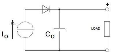
Conventional power supply circuit simplified, without PSINK
