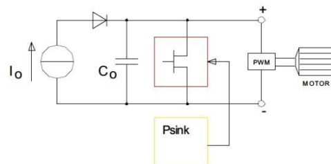
PSINK equipped power supply: absorbs breaking energy
