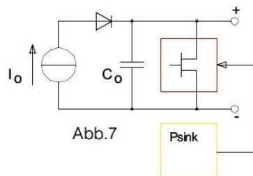
PSINK equipped power supply
