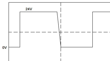
Latency of PSINK equipped power supply
