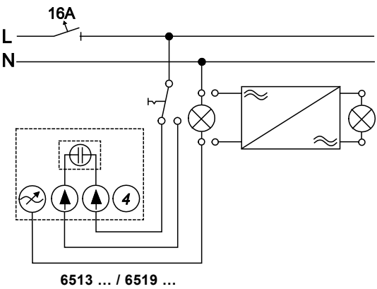
Fig. 3: Dimmer in two-way circuit
