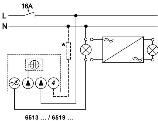
Fig. 4: Dimmer operation with voltage sensor
