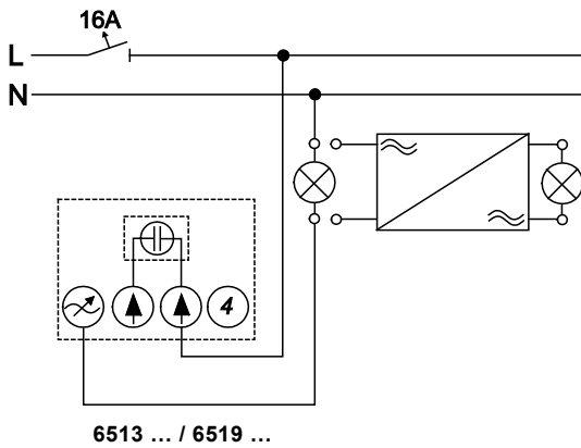
Fig. 2: Dimmer operation
