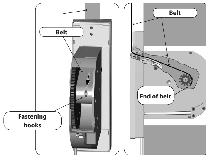
Belt path in RolloTron Standard
