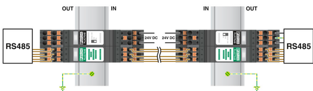
Application drawing
