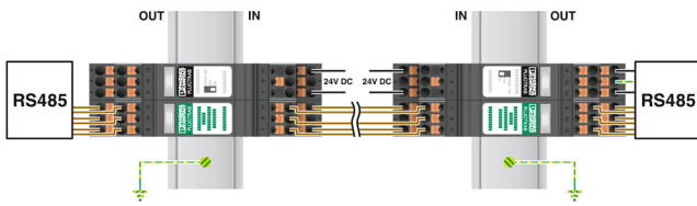
Application drawing
