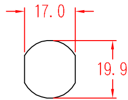
MOUNTING HOLE
