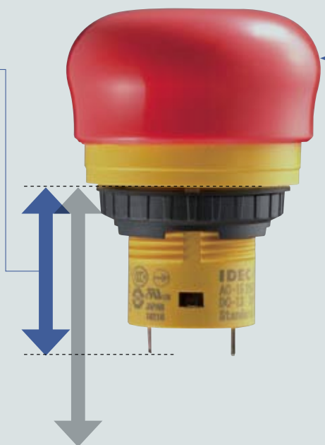
27.9 mm Conventional emergency stop switch with short depth behind the panel
