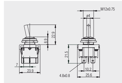
Quick-connect terminal 4.8 basic types 1822 and 1824
