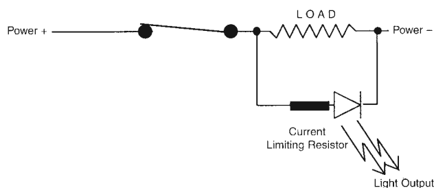
Figure 19. Wiring Diagram 4
