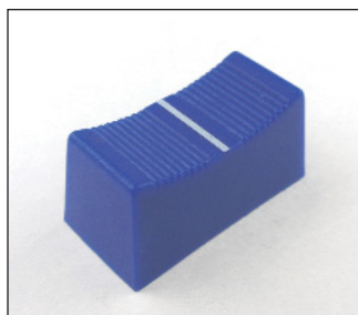
CP3265 CS/1A BLUE Length: 23mm Width: 11mm Height: 11mm For 4mm. shaft - Type A
