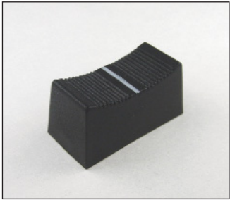
CP3260 CS/1A BLACK Length: 23mm Width: 11mm Height: 11mm For 4mm. shaft - Type A
