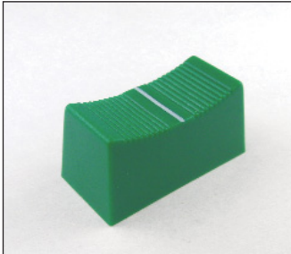
CP3270 CS/1A GREEN Length: 23mm Width: 11mm Height: 11mm For 4mm. shaft - Type A
