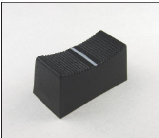
CP3261 CS/1B BLACK Length: 23mm Width: 11mm Height: 11mm For 4mm. shaft - Type B
