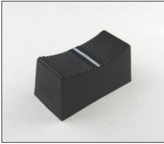
CP3155 CS/1 BLACK Length: 23mm Width: 11mm Height: 11mm For 6/8mm shaft
