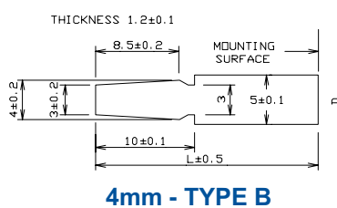
CP3193 CS/2B BLACK Length: 20mm Width: 14mm Height: 13mm For 4mm shaft - Type B
