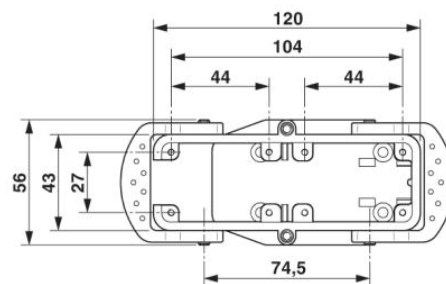
Dimensional drawing, a = 120 mm
