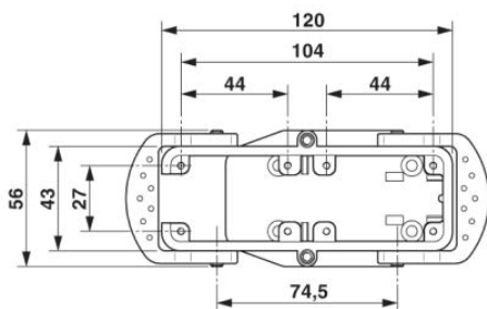
Dimensional drawing top view
