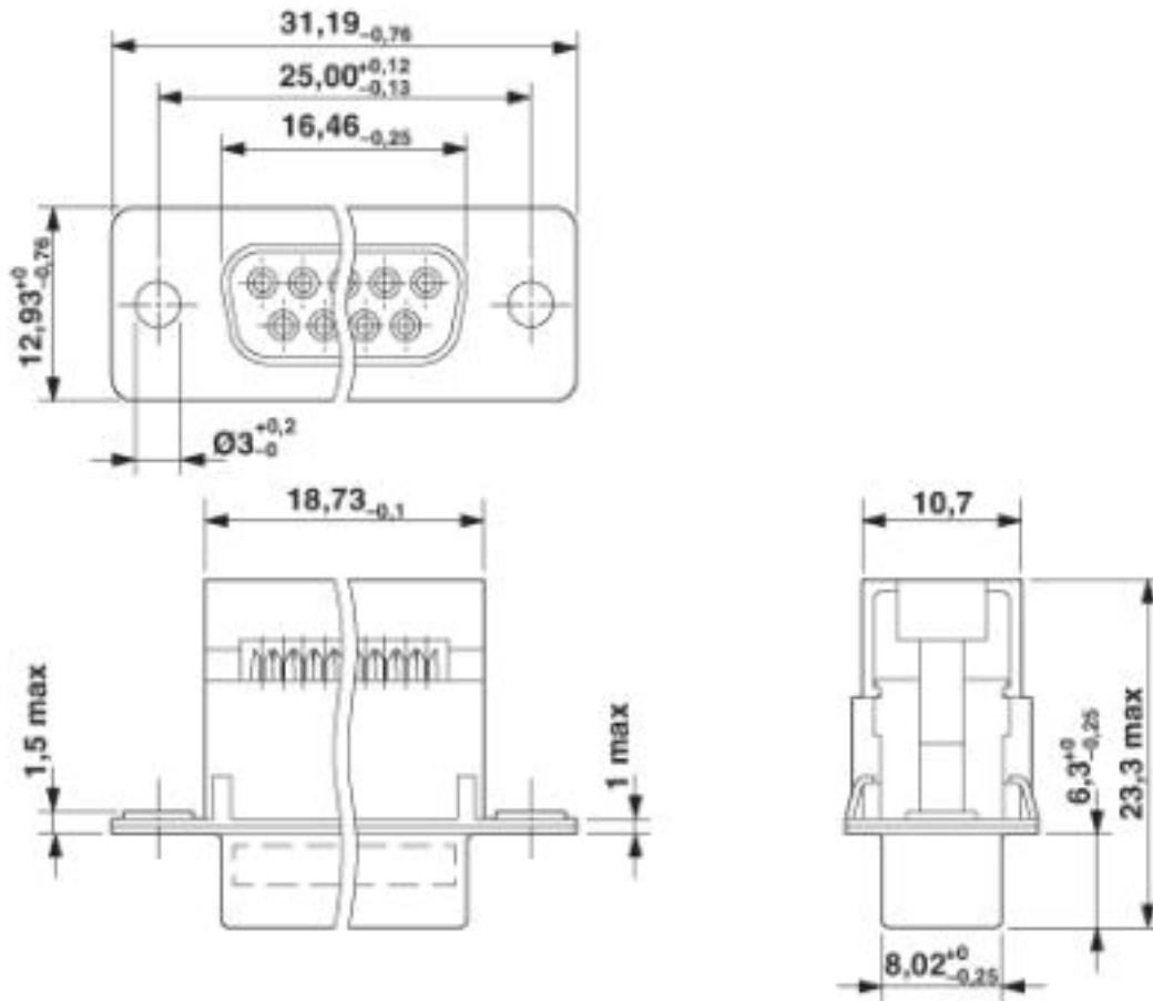
D-SUB contact insert
