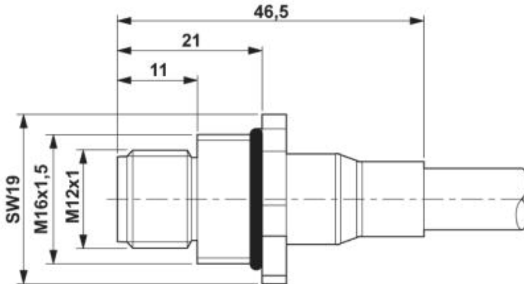
M12 flush-type plug
