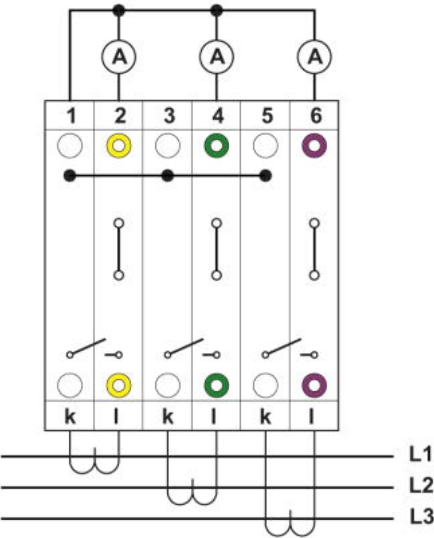
Connection diagram
