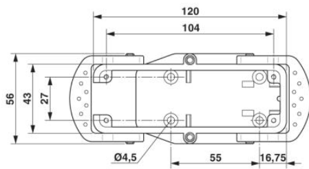
Dimensional drawing top view
