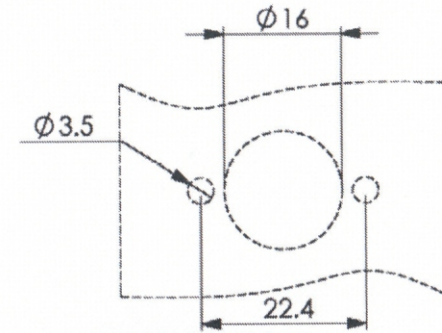
THROUGH HOLE DIMENSIONS
