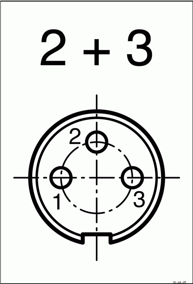
Contact arrangement
