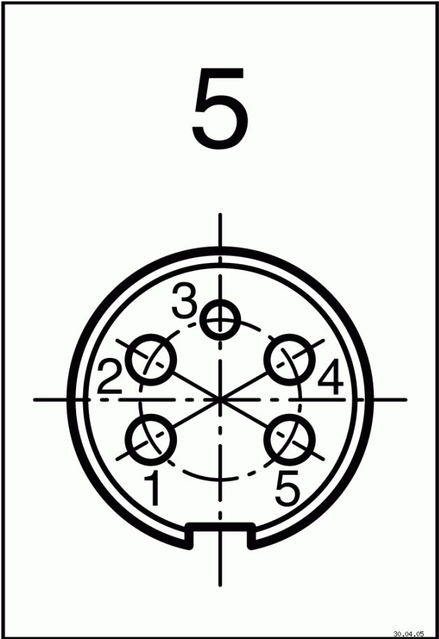
Contact arrangement
