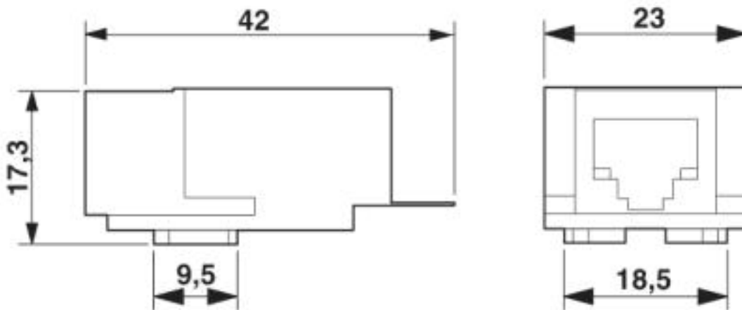
RJ45 socket insert
