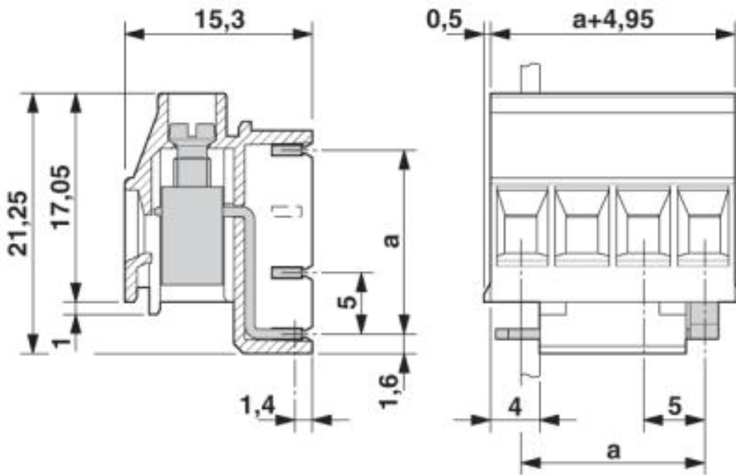
Dimensioned drawing
