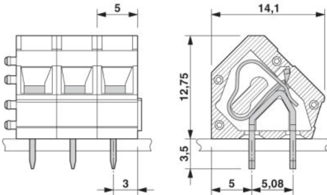
Dimensioned drawing
