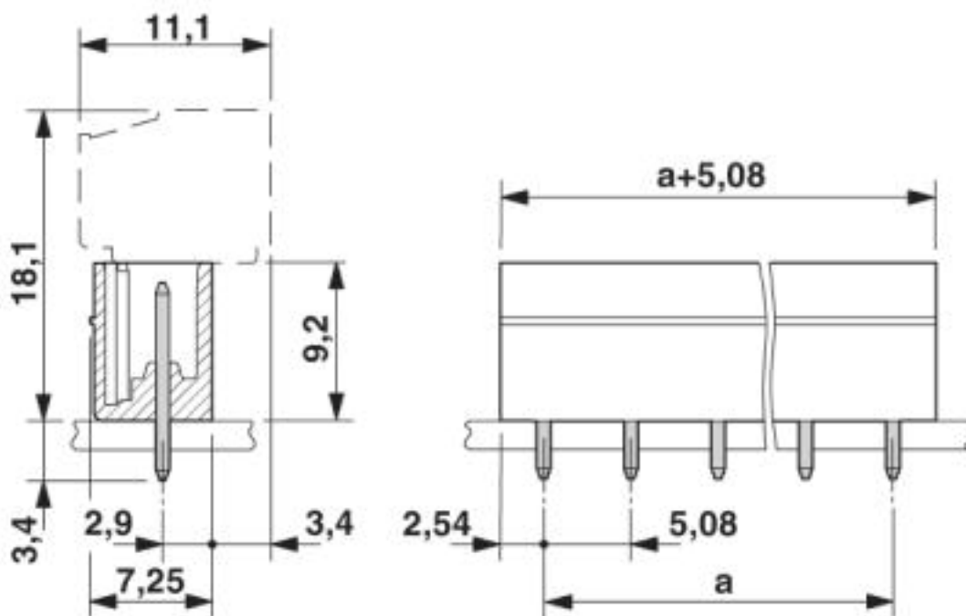
Dimensioned drawing
