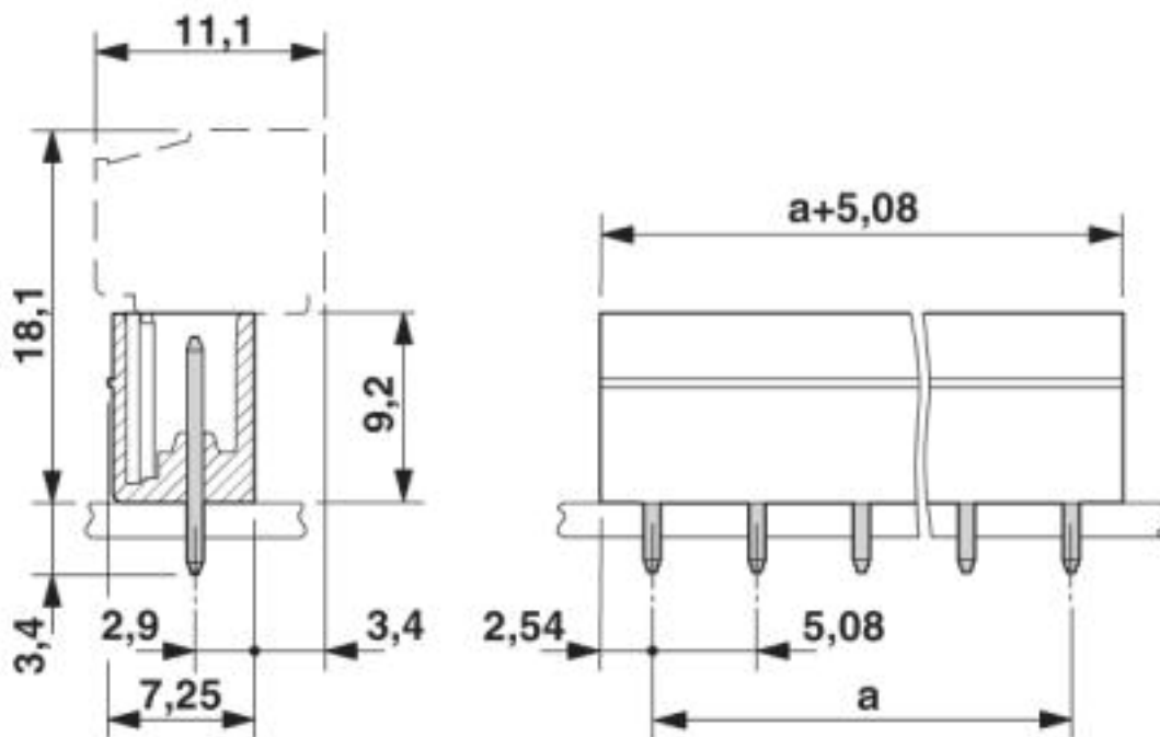
Dimensioned drawing
