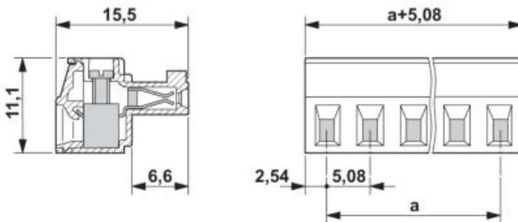
Dimensioned drawing
