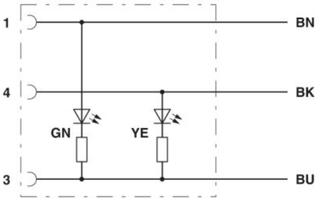
Contact assignment of M8 socket with 2 LEDs
