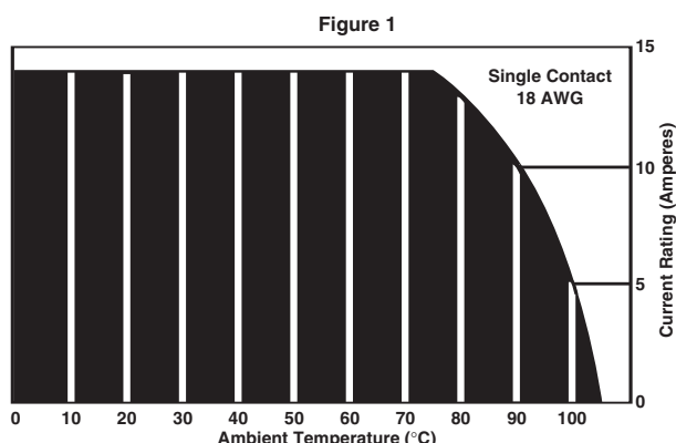
Graph shows the relationship between base current, ambient temperature, and contact T-rise.
