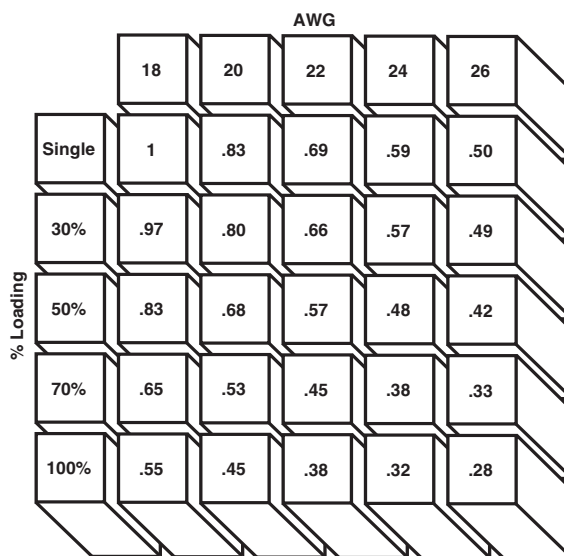
Rating factors allow the base current to be adjusted for various connector loading and wire sizes.
