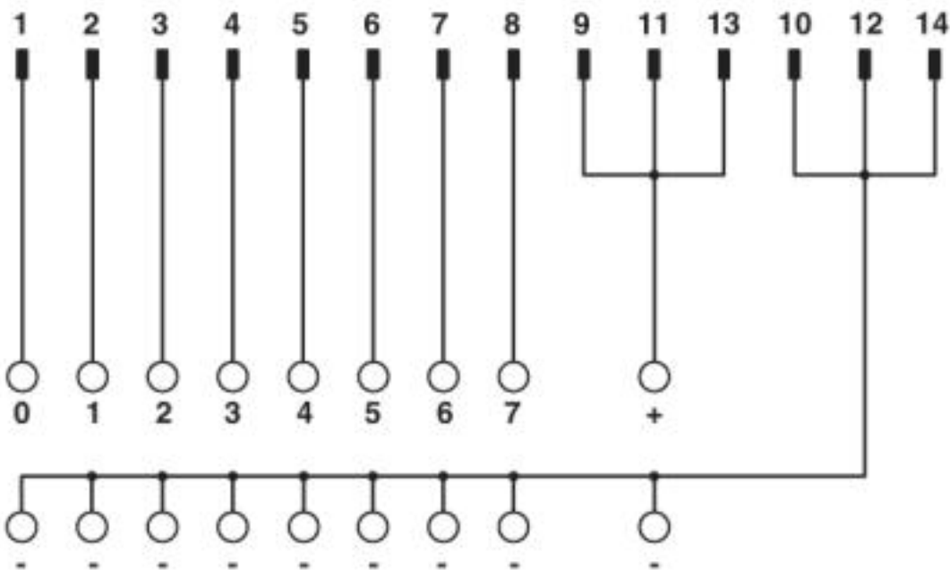
Connection scheme: FLKM 14/8M/PLC
