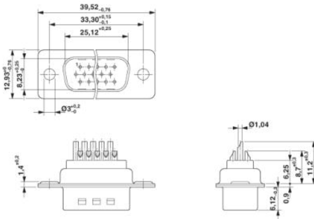
D-SUB contact insert
