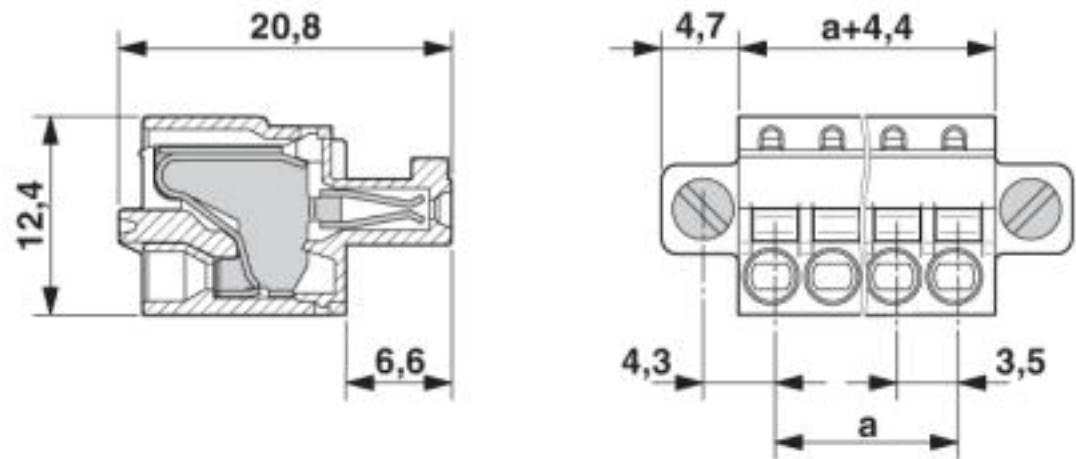
Dimensioned drawing
