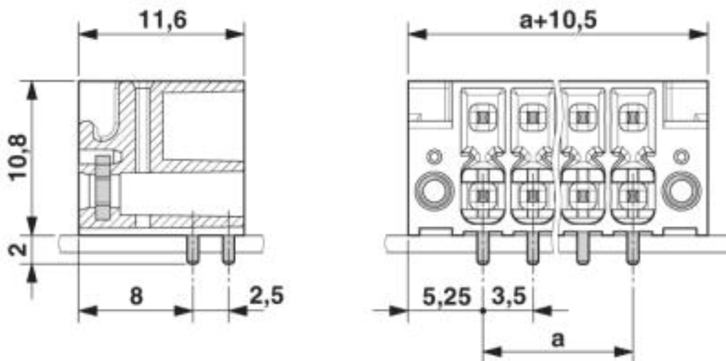
Dimensioned drawing
