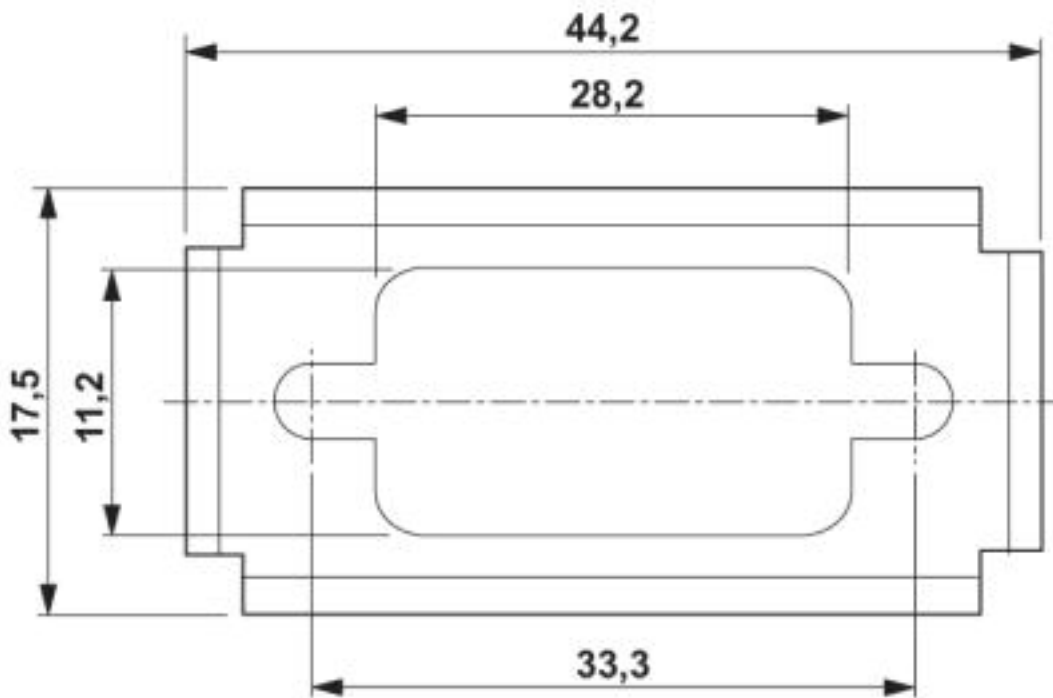
D-SUB EMC shroud
