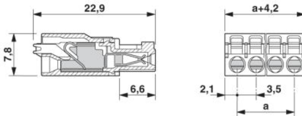
Dimensioned drawing
