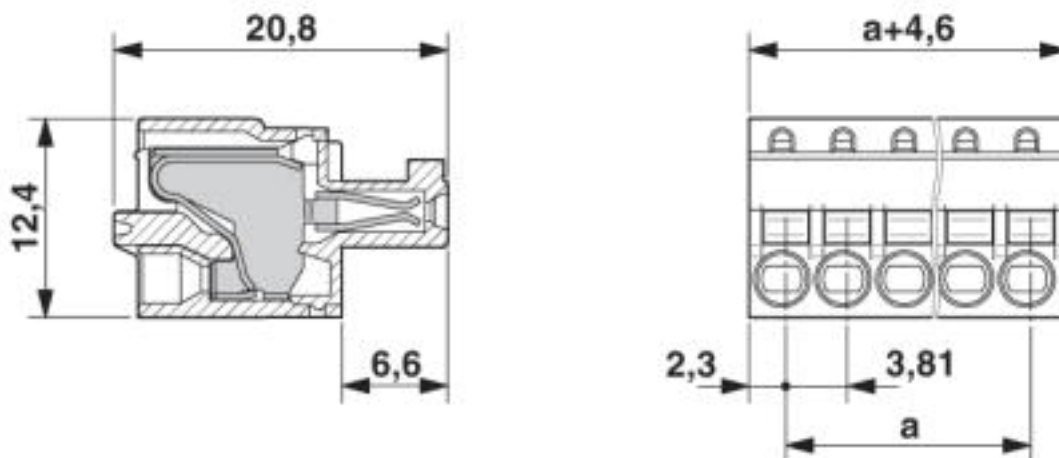
Dimensioned drawing
