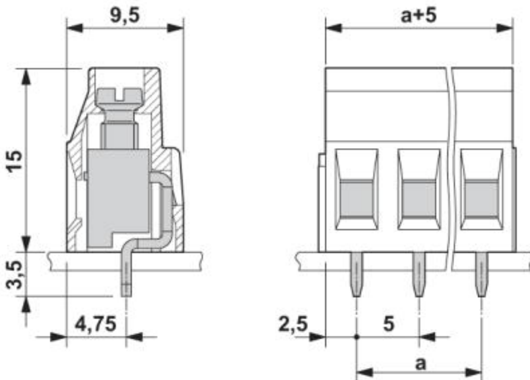
Dimensioned drawing
