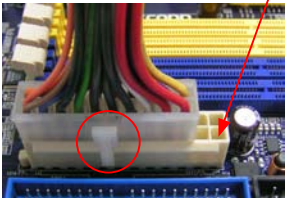
20-Pin Power
