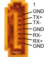
SATA_1/2/3/4/5/6
