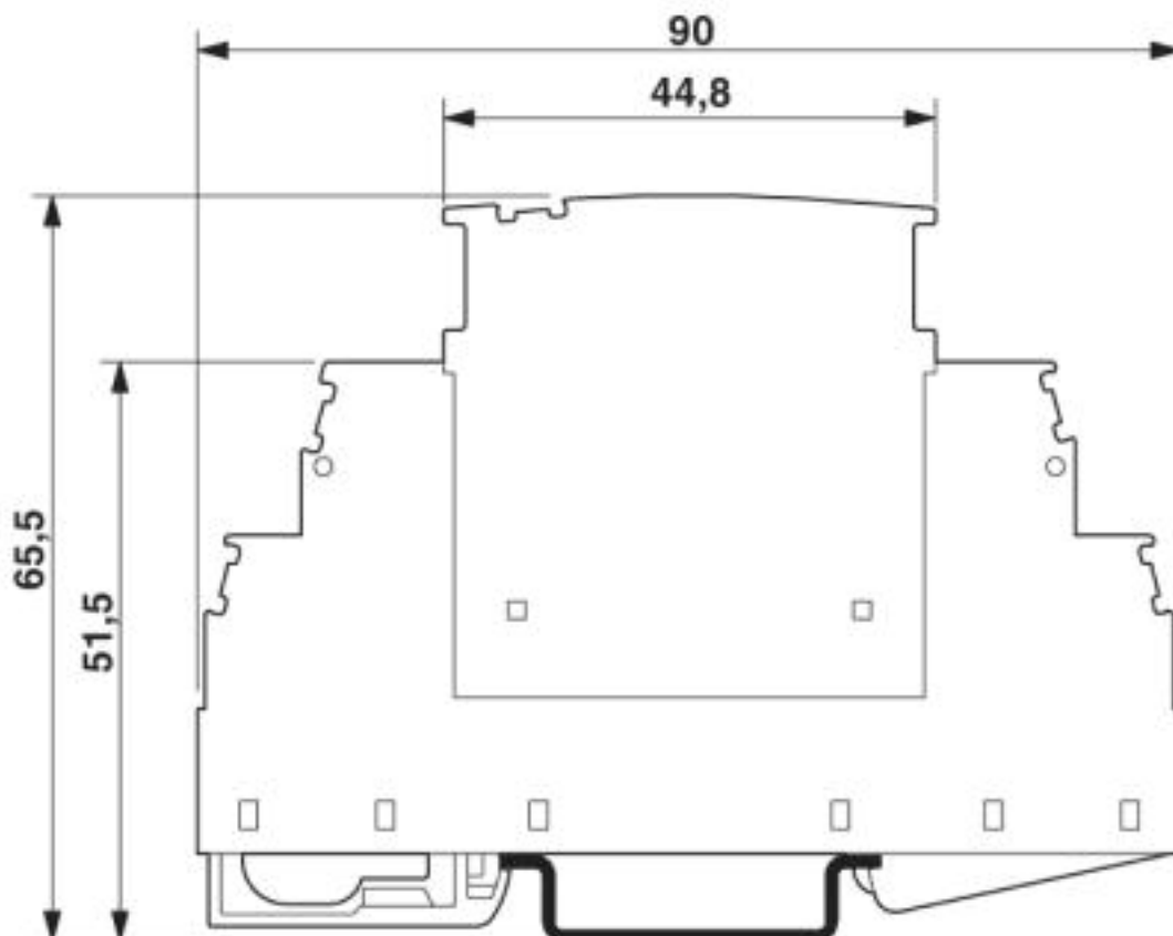
Dimensioned drawing
