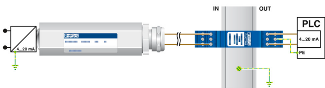
Application drawing
