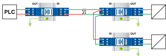
Application drawing
