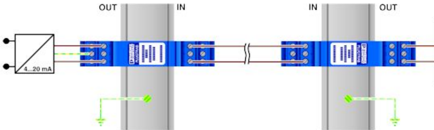
Application drawing
