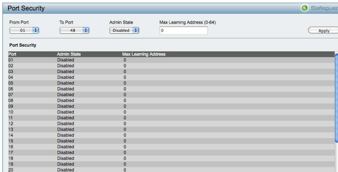
Figure 94 – Security > Port Security
