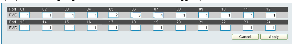
Figure 69 – Configuration > 802.1Q VLAN > Asymmetric VLAN – Assign PVID
