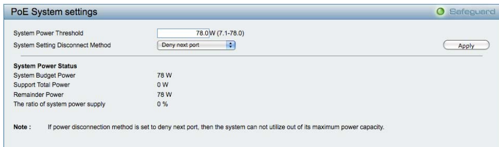
Figure 112 – PoE > PoE System Setting
