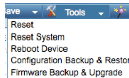
Figure 37 – Tool Menu
