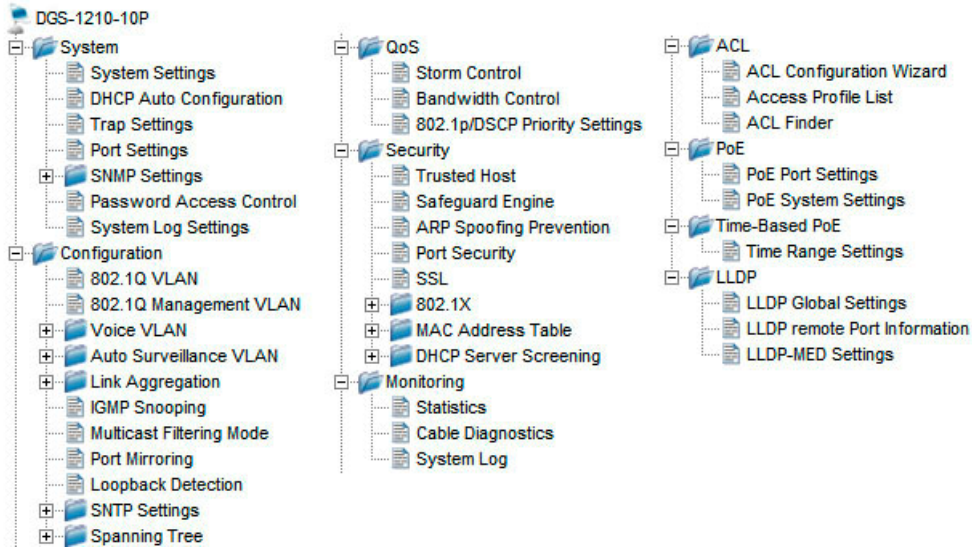
Figure 45 –Function Tree
