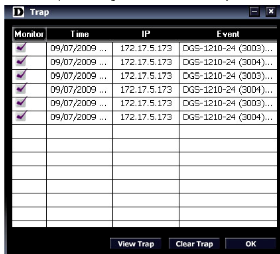
Figure 19 – SmartConsole Trap
