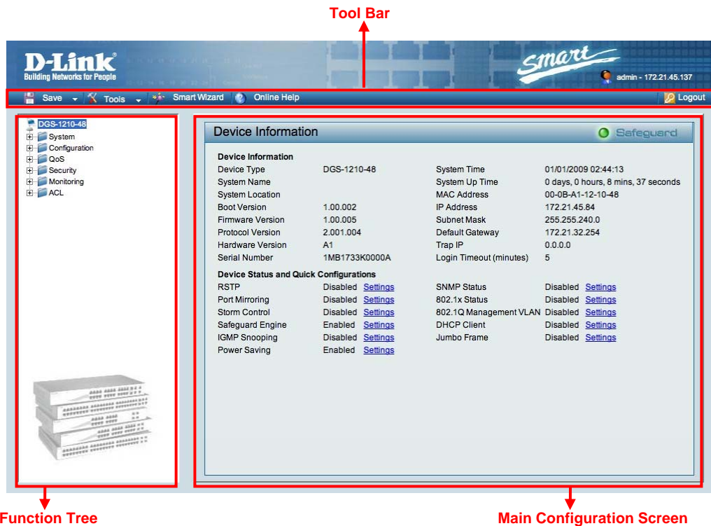
Figure 33 – Web-based Management
