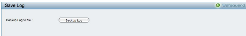
Figure 36 – Save Log
