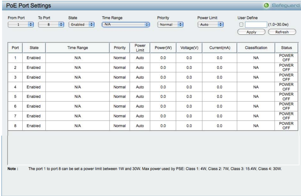
Figure 111 – PoE > PoE Port Setting
