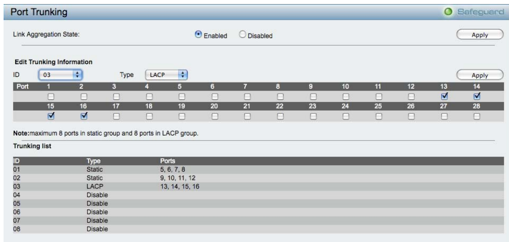
Figure 74 – Configuration > Link Aggregation > Port Trunking
