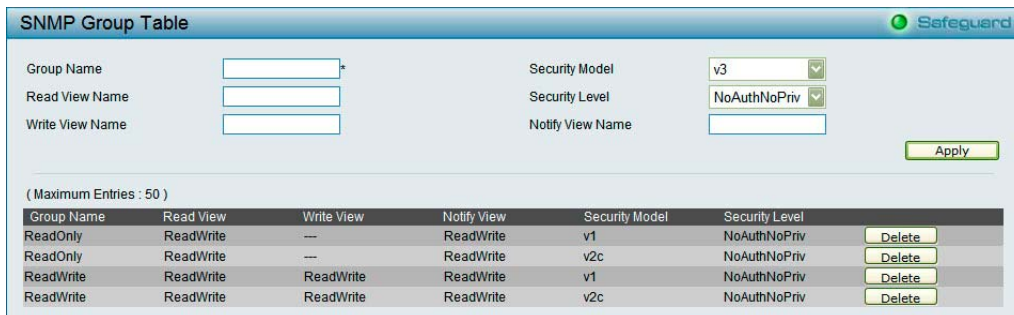
Figure 53 – System > SNMP Settings > SNMP Group Table
