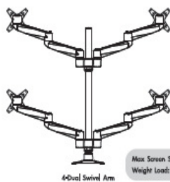
4-Dual Swivel Arm Max Screen Size: 27 inch Weight Load: total < 45kg
