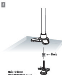
Hole: 10-40mm 鑿合的孔直徑: 10-40mm Thickness: 20-45mm 可夾持的厚度: 20-45mm
