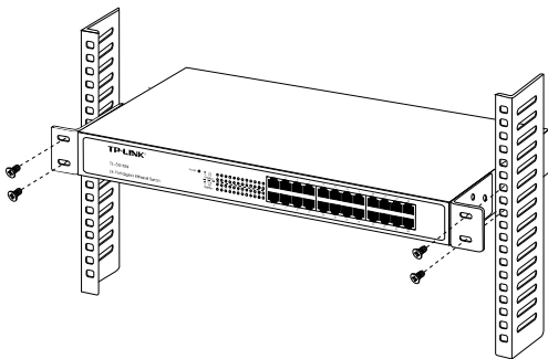
Figure 2-2 Fasten the Switch in the rack
