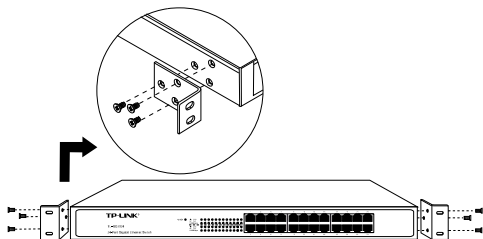
Figure 2-1 Rivet the "L" brackets onto the Switch
