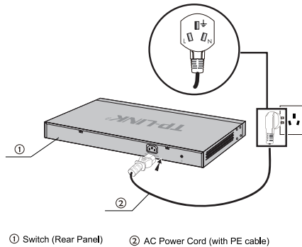
Figure 3-2 Connecting to the Ground
