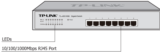
Figure 1-6 Front Panel of TL-SG1008
