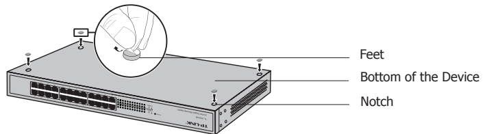
Figure 2-1 Desktop Installation
