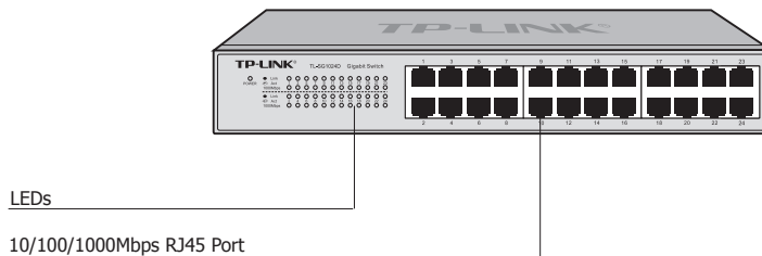
Figure 1-3 Front Panel of TL-SG1024D
