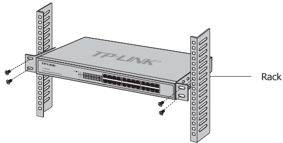
Figure 2-3 Rack Installation
