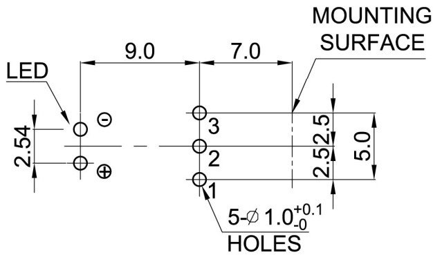
P.W.B MOUNTING DETAIL TOLERANCES ±0.1 VIEWED FROM MOUNTING SIDE P.C.B t=1.6
