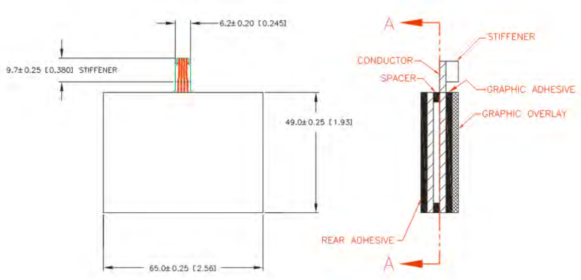
Figure 9: VersaPad Sensor
