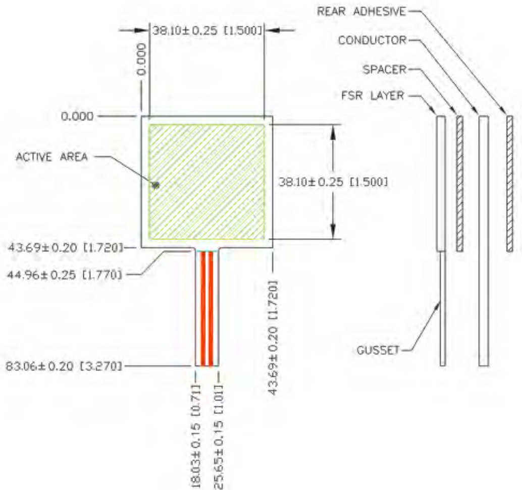
Figure 7: Model 406 Square FSR
