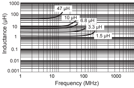
Typical Ls vs Frequency (f)
